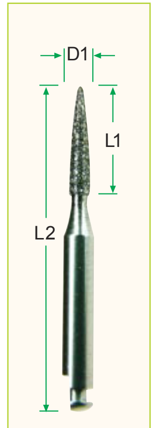
RA/CA -Dimensions
