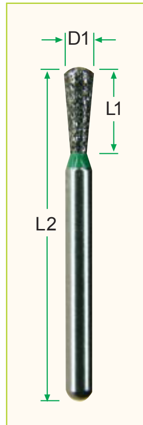
FG -Dimensions
